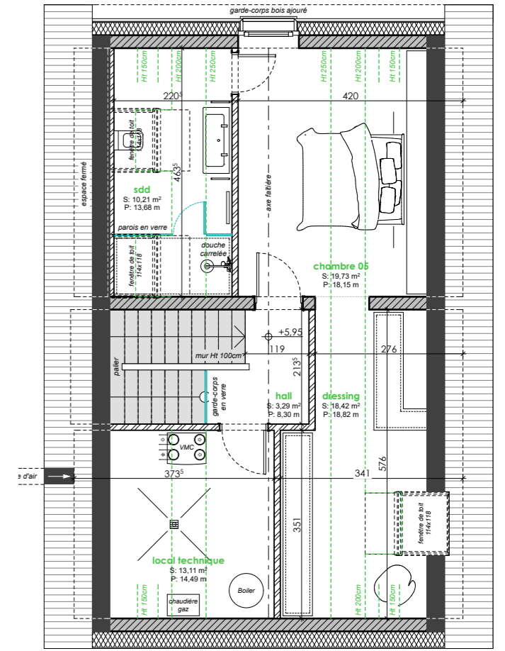
Combles
